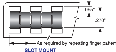
SLOT MOUNT
