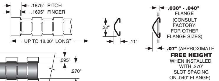
SLOT MOUNT
