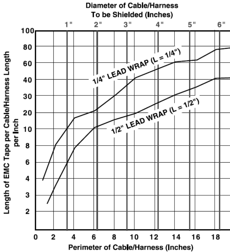
Tape Length vs Cable Size — Figure 2
