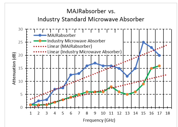
Figure #2 Attenuation (dB) vs. frequency (GHz)
